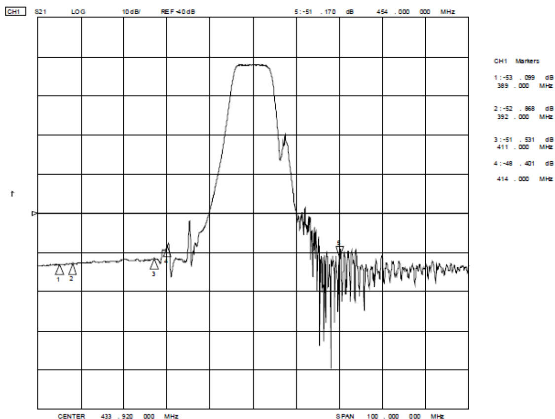
Fig.3 STR29RSH4 RF Front End SAW Filter Frequency Response
