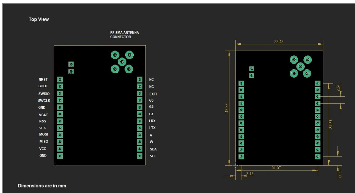
Fig.10 STR29RSH4 Pin and Size Diagram
