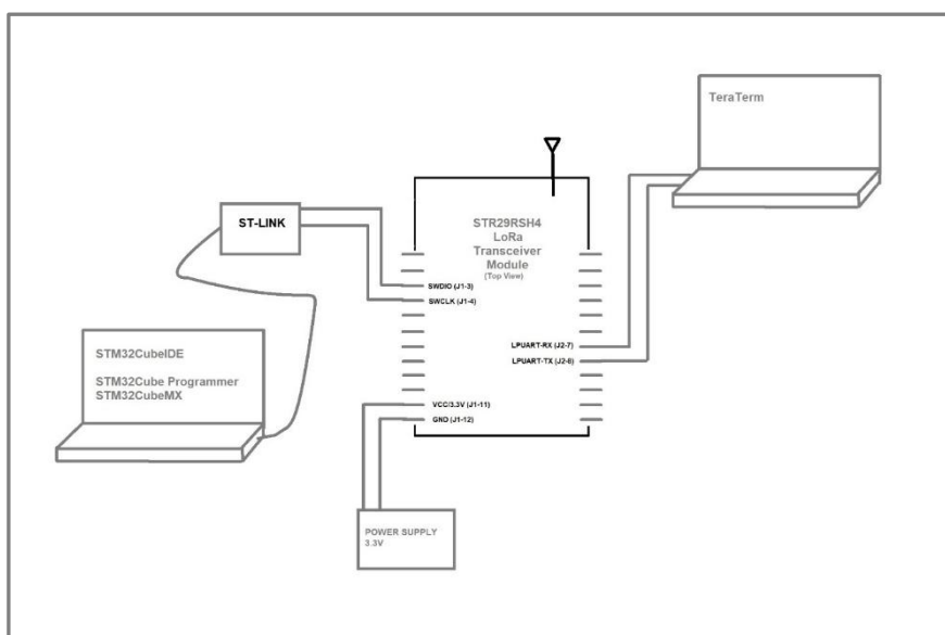
Fig.5 STR29RSH4 Code Development/Porting/Testing
