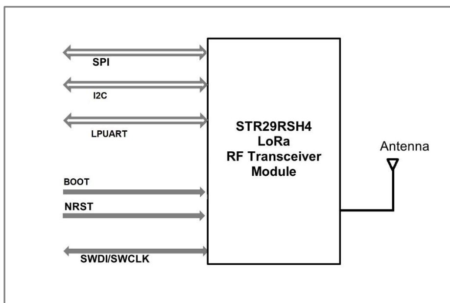
Fig.6 Interfacing STR29RSH4 to external units
