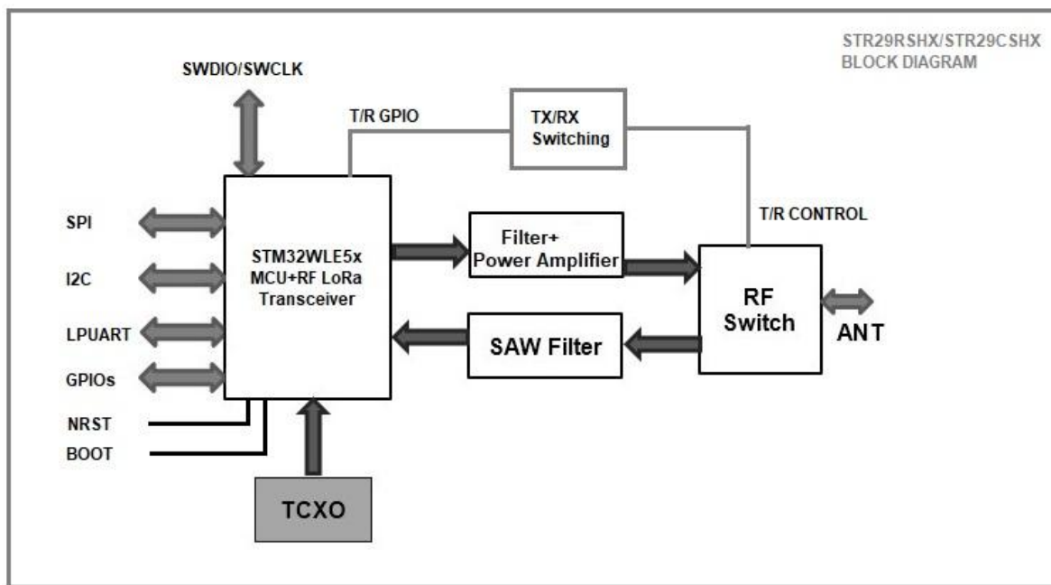
Fig.1 STR29RSH4 functional blocks and interconnections
