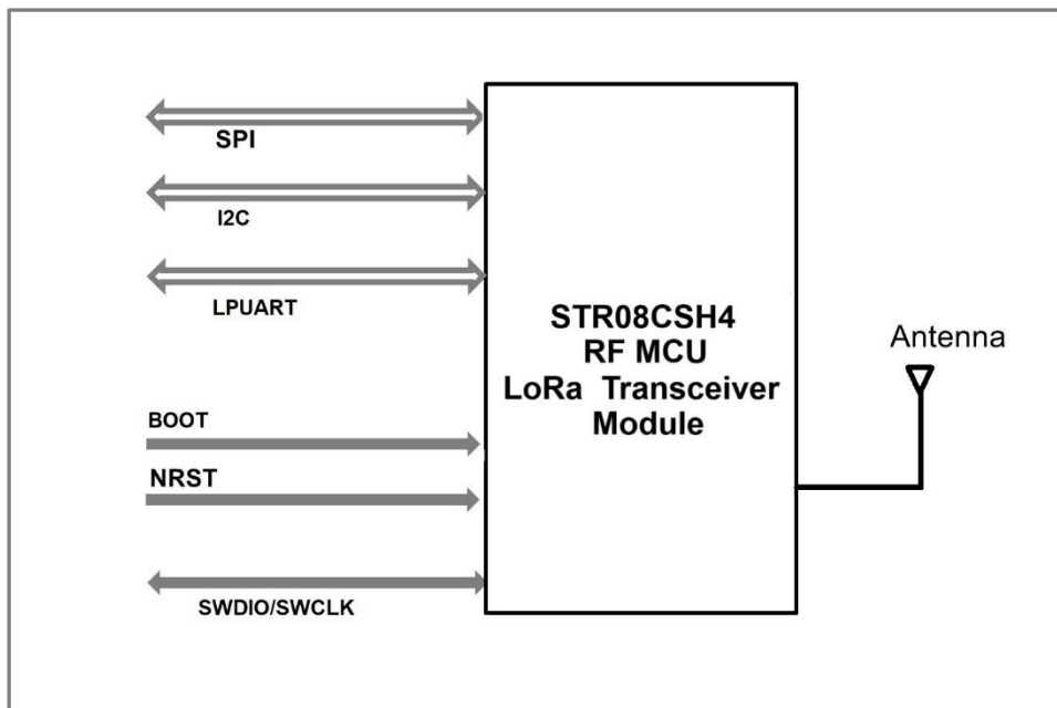
Fig.6 Interfacing STR08CSH4 to external units
