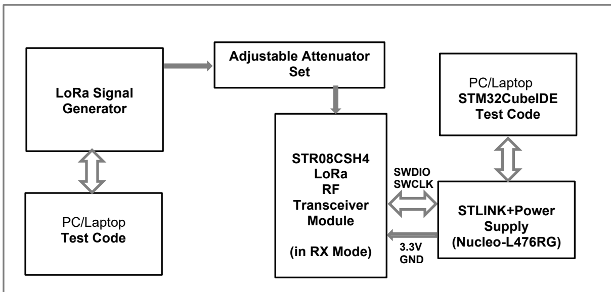
Fig.11 STR08CSH4 Receive Mode Test & Measurement Setup
