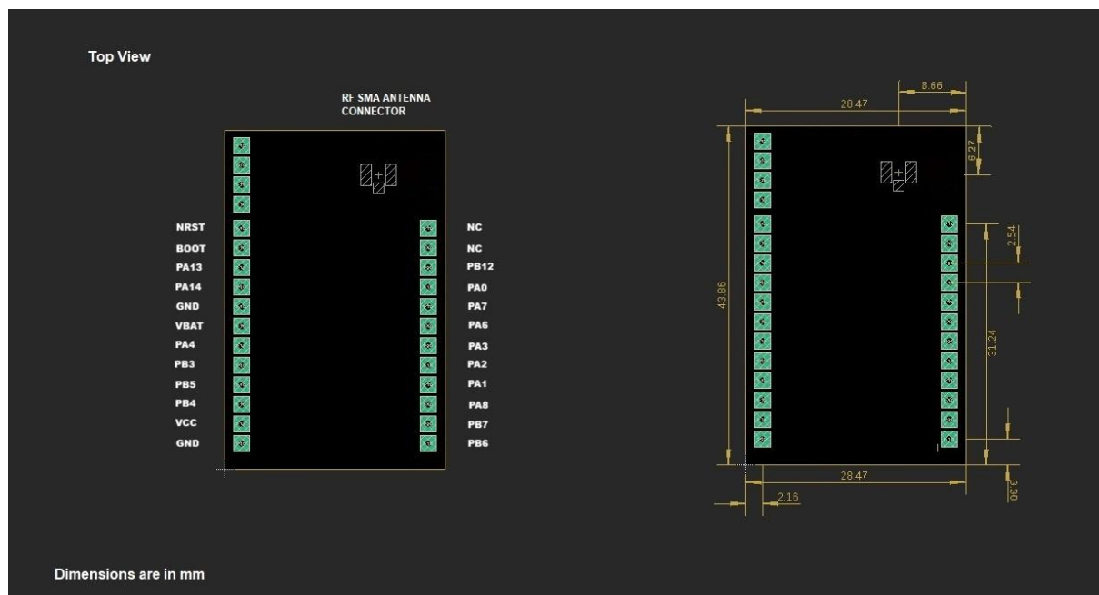
Fig.12 STR08CSH4 Pin and Size Diagram
