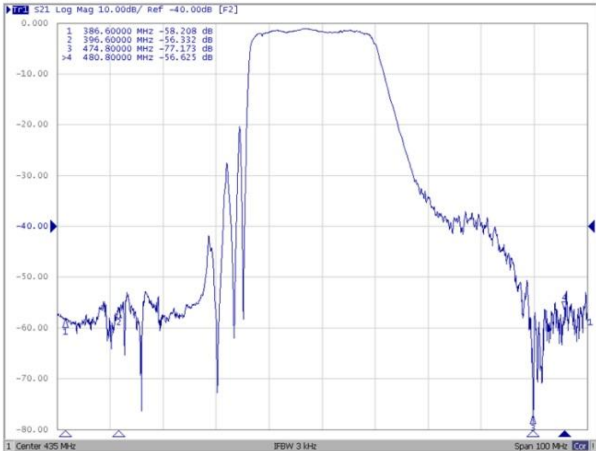
Fig.3 STR08CSH4 RF Frontend SAW Filter Frequency Response
