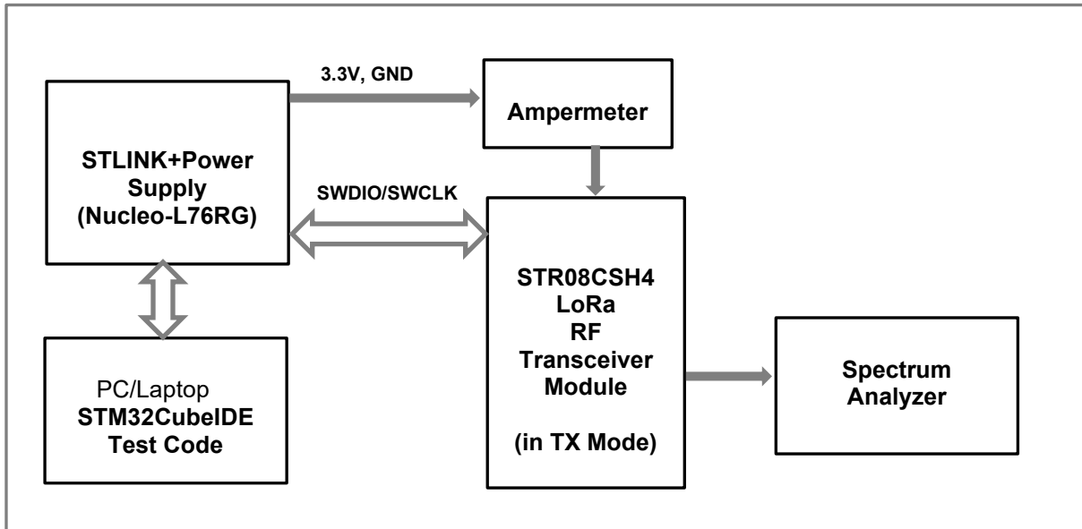
Fig.10 STR08CSH4 Transmit Mode Test & Measurement Setup
