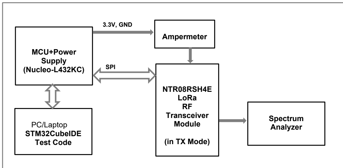
Fig.10 NTR08RSH4E Transmit Mode Test & Measurement Setup
