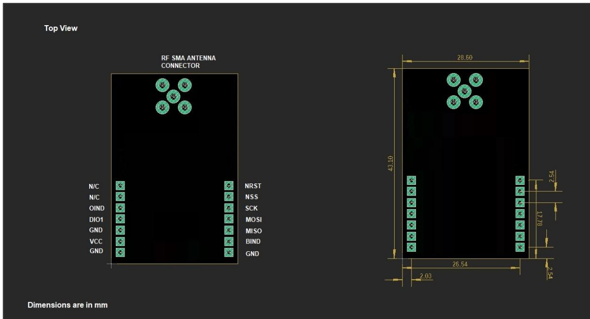
Fig.12 NTR08RSH4E Pin and Size Diagram
