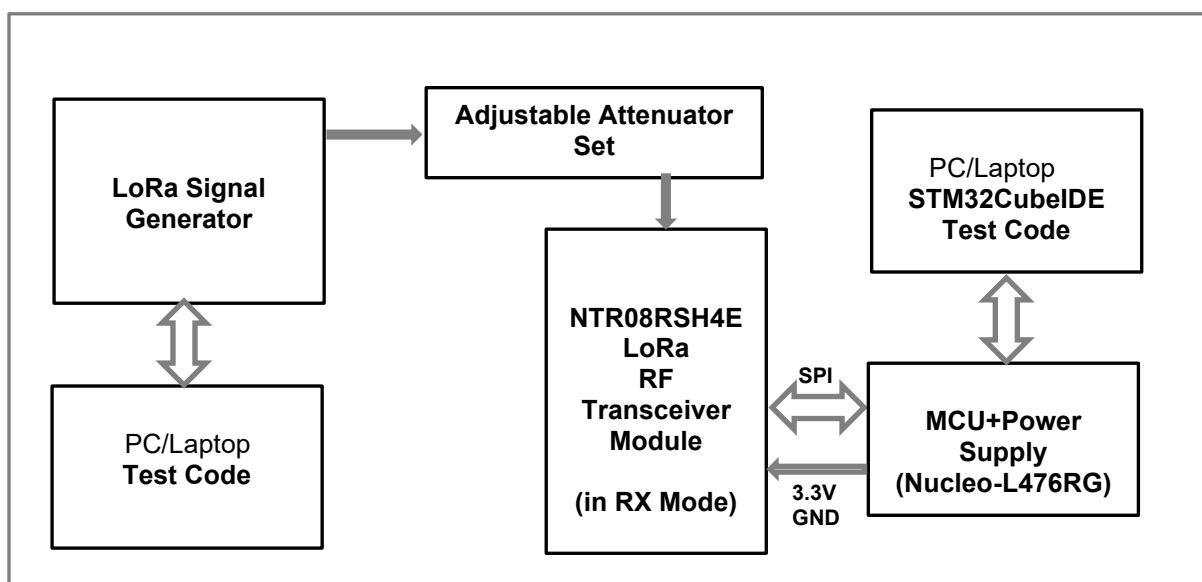
Fig.11 NTR08RSH4E Receive Mode Test & Measurement Setup
