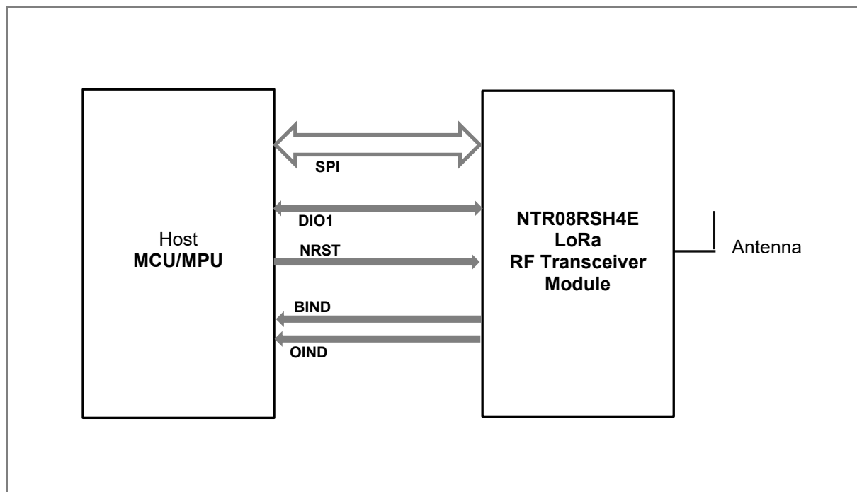
Fig.5 Interfacing NTR08RSH4E to MCU/MPU
