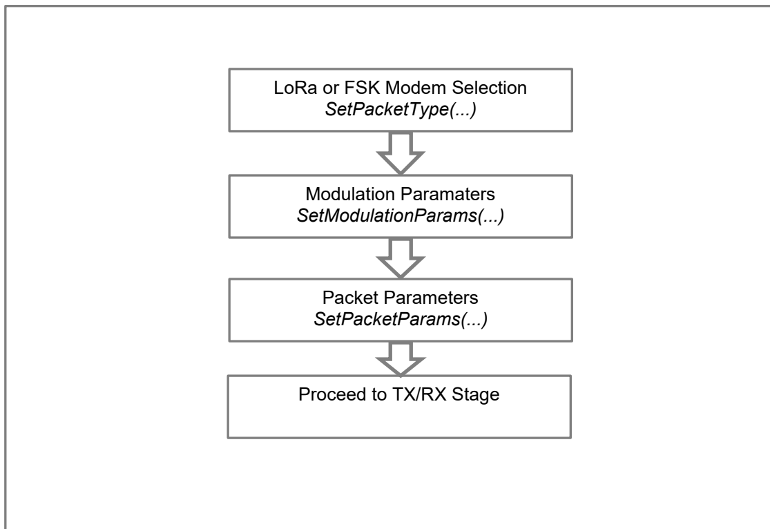
Fig.8 Configuration and Settings - Modem Selection, Modulation and Packet Parameters
