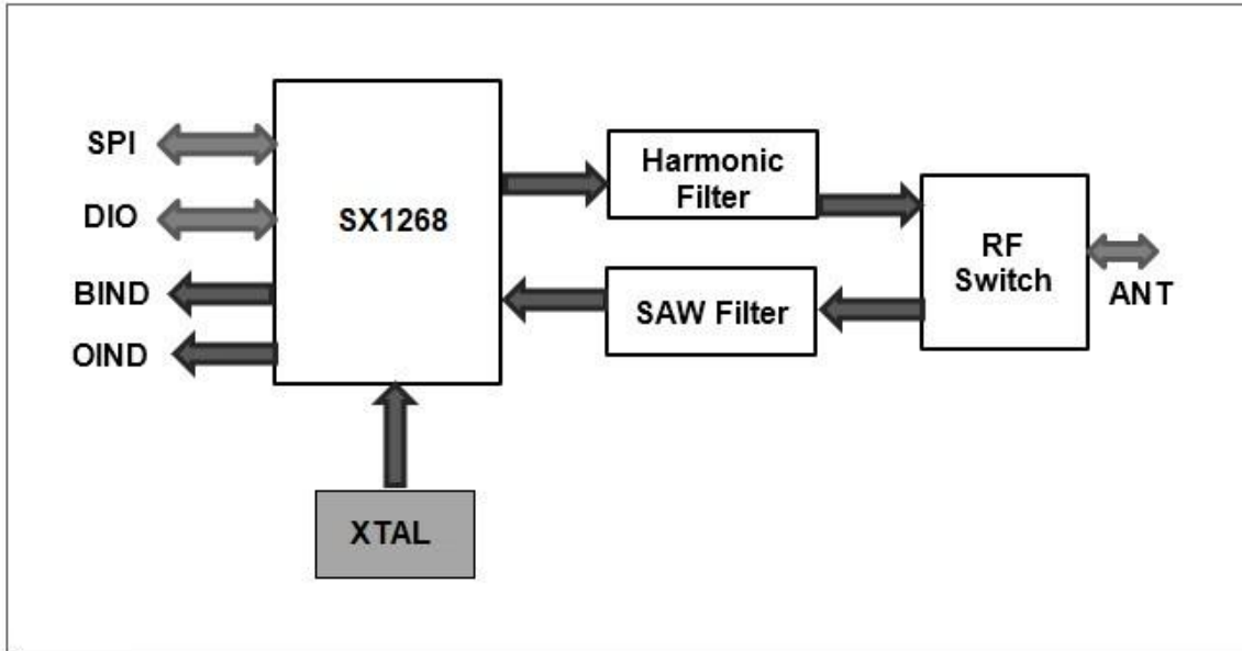
Fig.1 NTR08RSH4E functional blocks and interconnections
