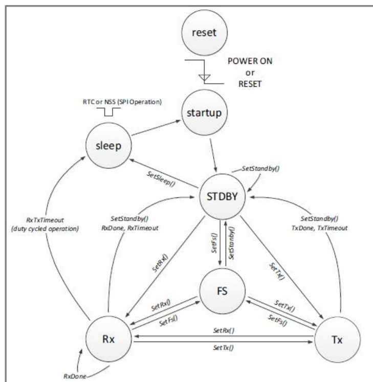
Fig.6 NTR08RSH4E Operational Modes
