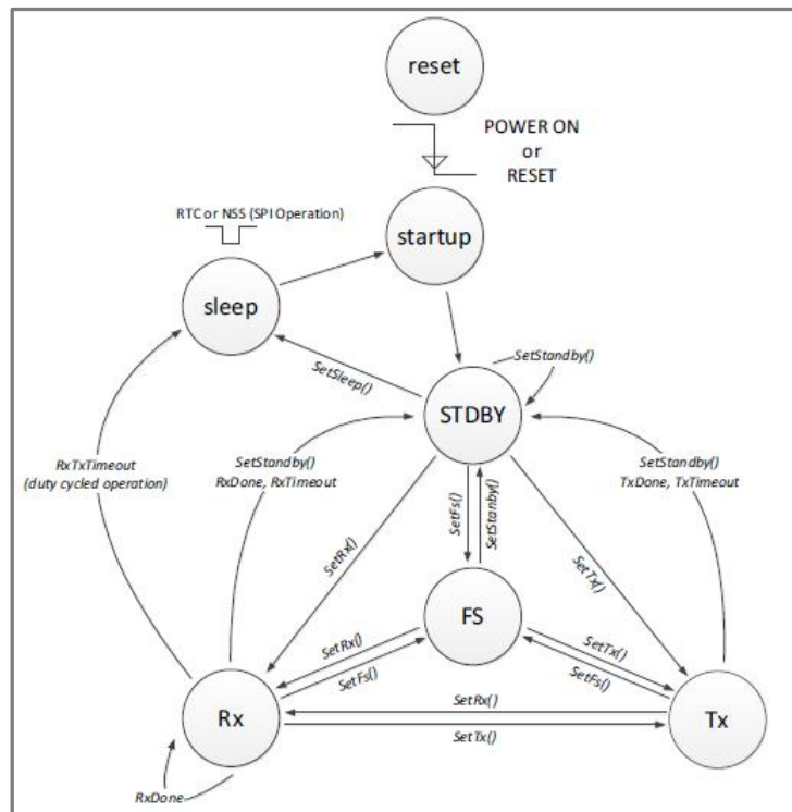
Fig.6 LTR26RSH3 Operational Modes
