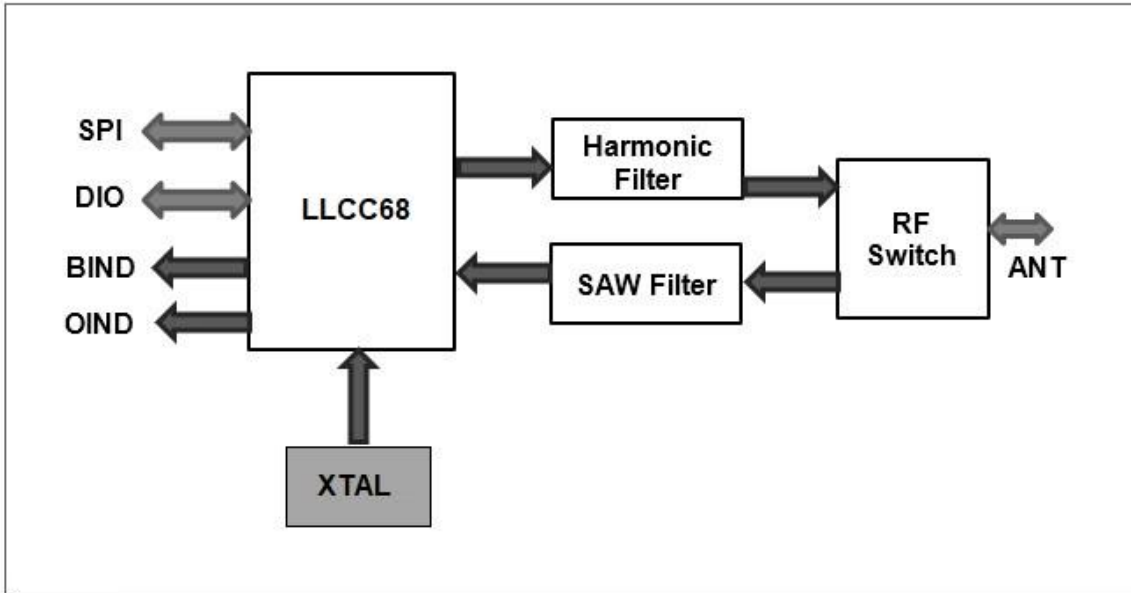
Fig.1 LTR26RSH3 functional blocks and interconnections
