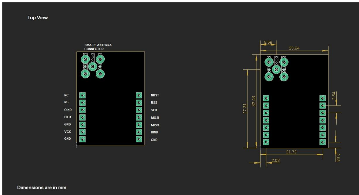
Fig.11 LTR26RSH3 Pin and Size Diagram
