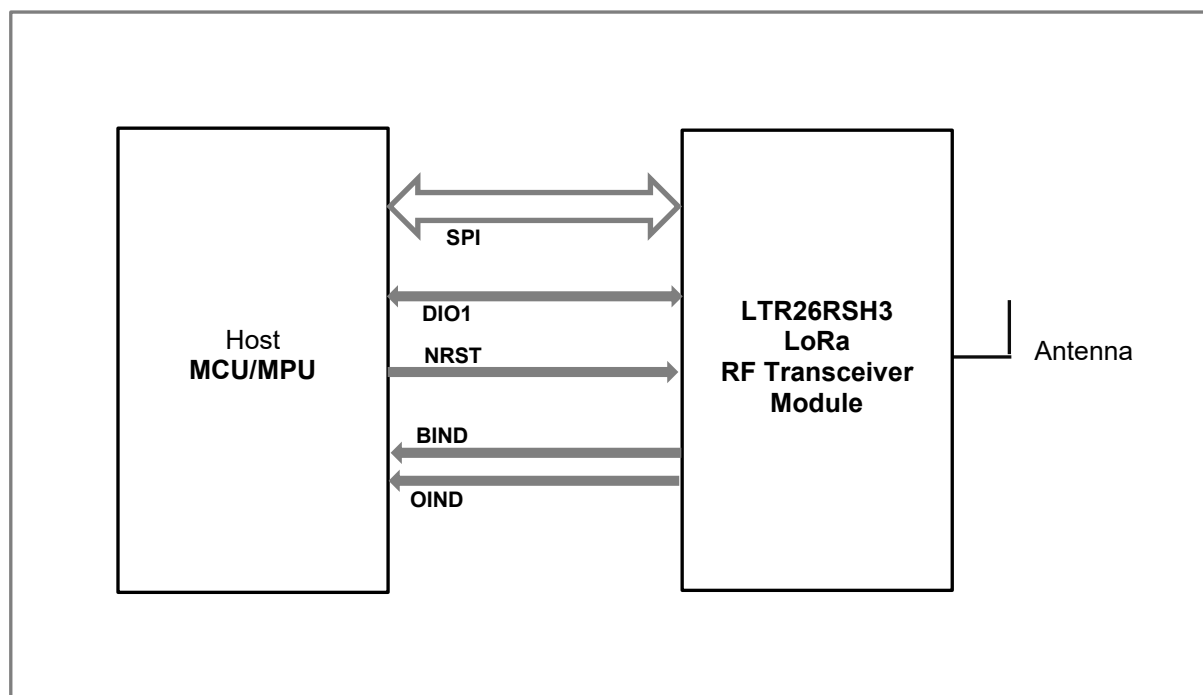
Fig.5 Interfacing LTR26RSH3 to MCU/MPU
