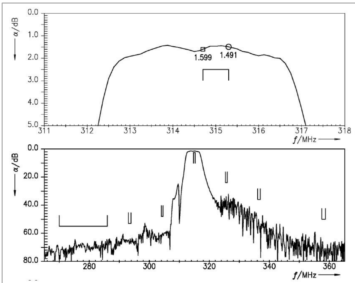
Fig.3 LTR26RSH3 RF Frontend SAW Filter Frequency Response
